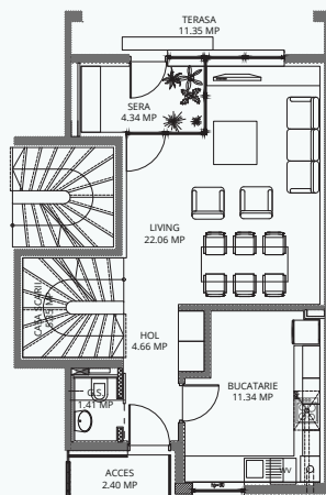
Parter ▲
